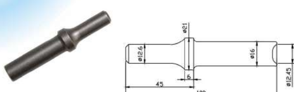
TP-2214 5/16" Rivet Caulking Chisel (Chisel Shank 12.6mm)
