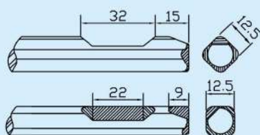
TP-2501 Moil Point Chisel
