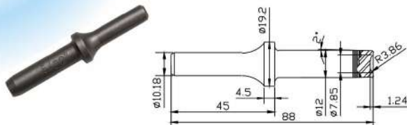
TP-2204 3/16" Rivet Caulking Chisel (Chisel Shank 10.18mm)
