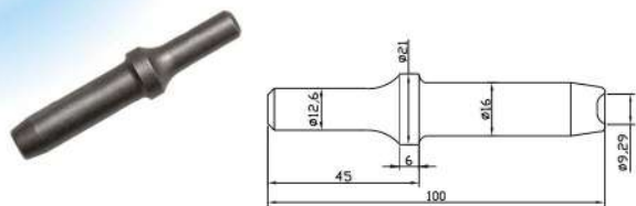
TP-2213 1/4" Rivet Caulking Chisel (Chisel Shank 12.6mm)
