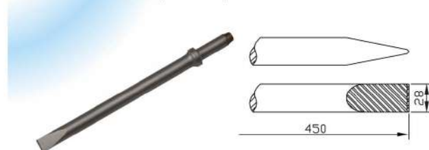
TP-2142 Flat Chisel (for At-2116)
