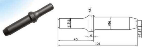
TP-2212 3/16" Rivet Caulking Chisel (Chisel Shank 12.6mm)
