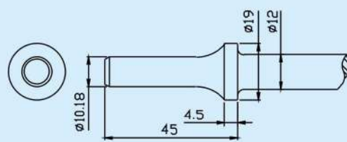
TP-2022 Flat chisel
