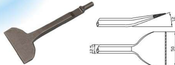
TP-2685 50mm Wide Bent Chisel
