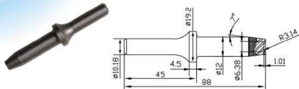
TP-2203 5/32" Rivet Caulking Chisel (Chisel Shank 10.18mm)
