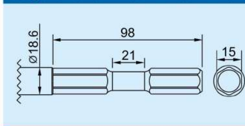
Scraper Chisel for AT-2506 AT-2506L AT-2513
