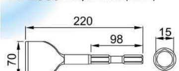
TP-2508 Scraper Chisel (70mm)
