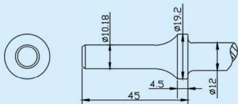
TP-2201 3/32" Rivet Caulking Chisel (Chisel Shank 10.18mm)
