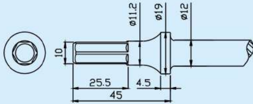
TP-2021 Point chisel
