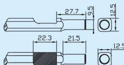
TP-2681 Moil Point Chisel
