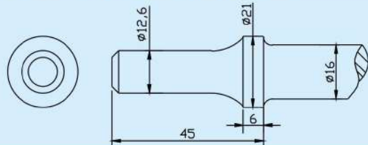
TP-2211 5/32" Rivet Caulking Chisel (Chisel Shank 12.6mm)
