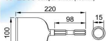
TP-2509 Scraper Chisel (100mm)
