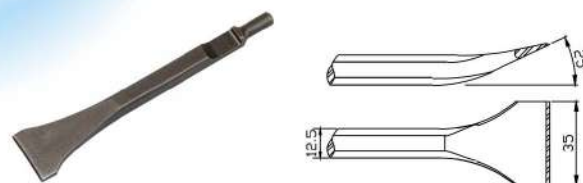
TP-2684 40mm Wide Cutting Chisel
