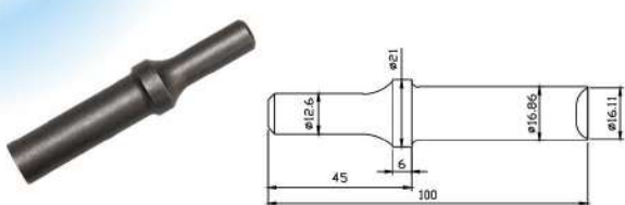
TP-2215 1-1/4" Rivet Caulking Chisel (Chisel Shank 12.6mm)
