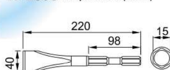
TP-2506 Scraper Chisel (40mm)
