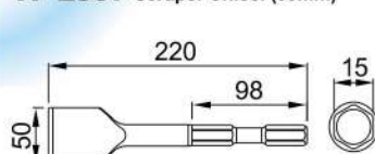
TP-2507 Scraper Chisel (50mm)
