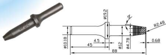
TP-2202 1/8" Rivet Caulking Chisel (Chisel Shank 10.18mm)
