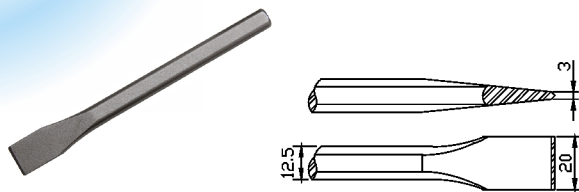
TP-2503 35mm Wide Bent Chisel
