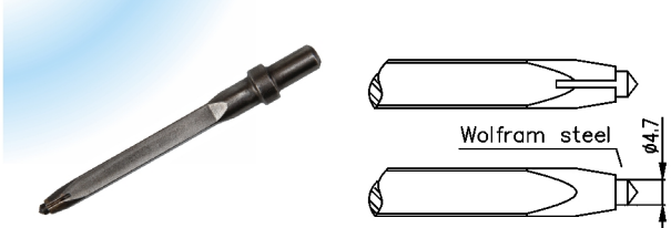
TP-2513 Moil Point Chisel (for AT-2511)
