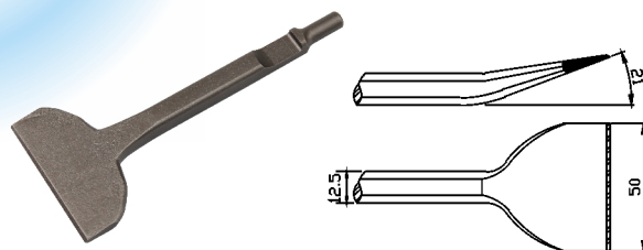
TP-2685 50mm Wide Bent Chisel
