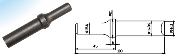
TP-2215 1-1/4" Rivet Caulking Chisel (Chisel Shank 12.6mm)
