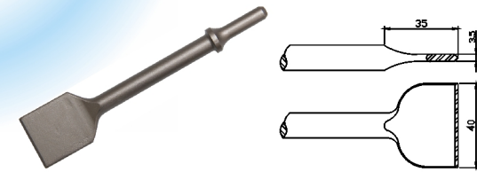
TP-2036 40mm Moon-shape chisel
