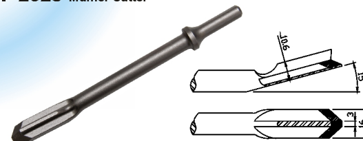
TP-2028 Muffler Cutter
