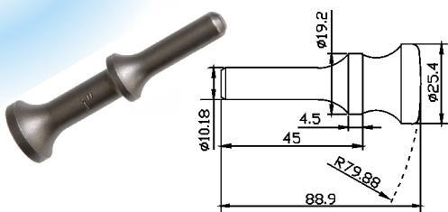
TP-2205 1" Rivet Caulking Chisel (Chisel Shank 10.18mm)
