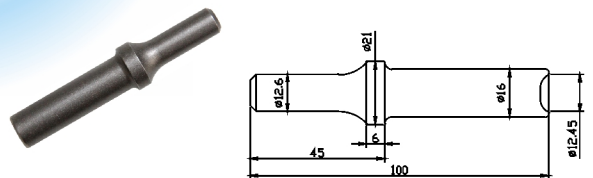
TP-2214 5/16" Rivet Caulking Chisel (Chisel Shank 12.6mm)
