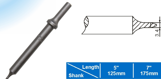
TP-2055 Rivet Removing Punch
