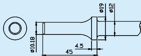
TP-2022 Flat chisel
