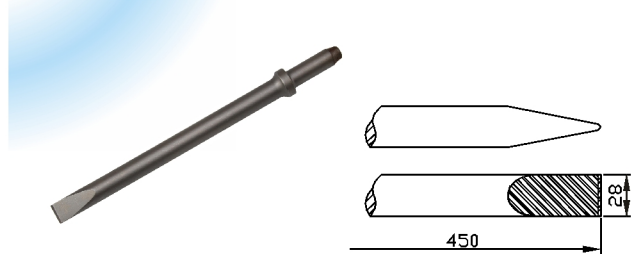
TP-2142 Flat Chisel (for At-2116)
