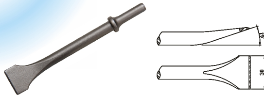
TP-2031 30mm Wide Bent Chisel
