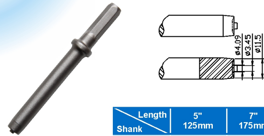
TP-2053 Hollow rivet Chisel 6mm
