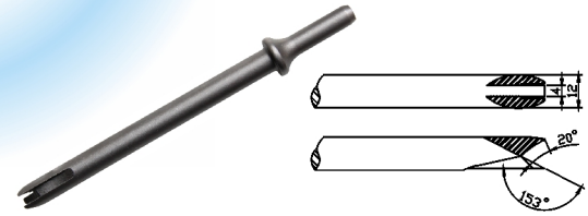
TP-2037 Sheet Metal Cutter
