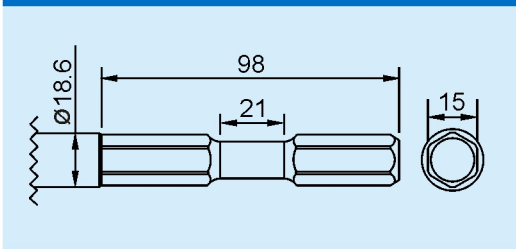
Scraper Chisel for AT-2506 AT-2506L AT-2513
