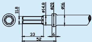
TP-2121 Moil Point
