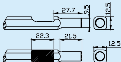
TP-2681 Moil Point Chisel
