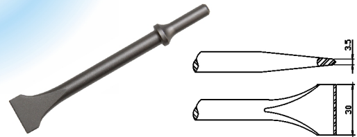
TP-2030 30mm Wide Flat Chisel
