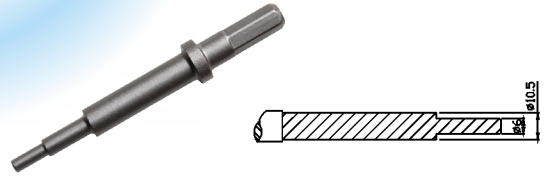
TP-2041 Wide Guide Driver Tool
