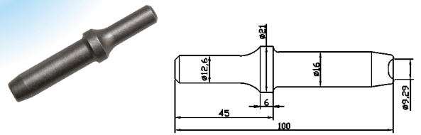
TP-2213 1/4" Rivet Caulking Chisel (Chisel Shank 12.6mm)
