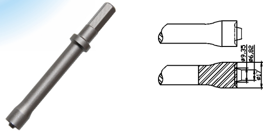
TP-2051 Hollow rivet Chisel 10mm
