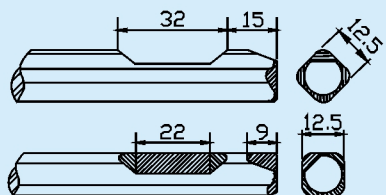
TP-2501 Moil Point Chisel
