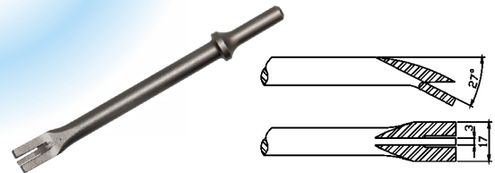
TP-2045 Shred Metal Trimmer
