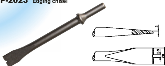
TP-2023 Edging chisel
