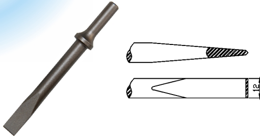
TP-2050 12mm Wide Cutting Chisel
