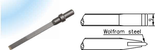
TP-2514 Flat Chisel (for AT-2511)
