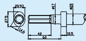
TP-2101 Moil Point
