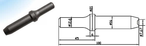
TP-2212 3/16" Rivet Caulking Chisel (Chisel Shank 12.6mm)
