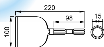
TP-2509 Scraper Chisel (100mm)
