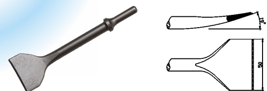
TP-2039 50mm Wide Cutting Chisel
