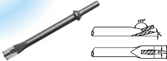
TP-2029 Sheet Metal Trimmer
