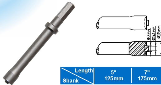
TP-2052 Hollow rivet Chisel 8mm
