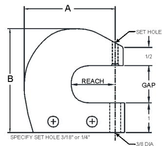
D TYPE (Longeron Yoke)
